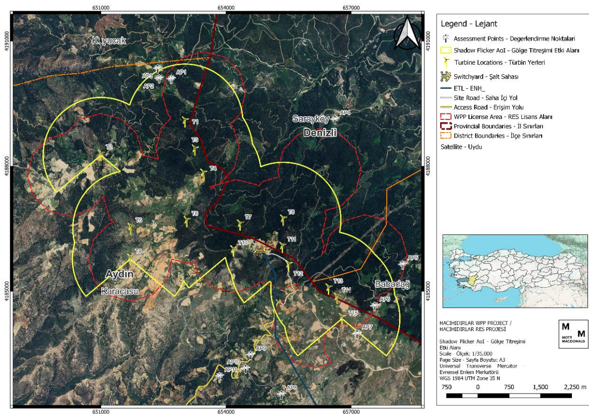
Figure 3.3: Shadow Flicker AoI ( \theta=260^\circ )
