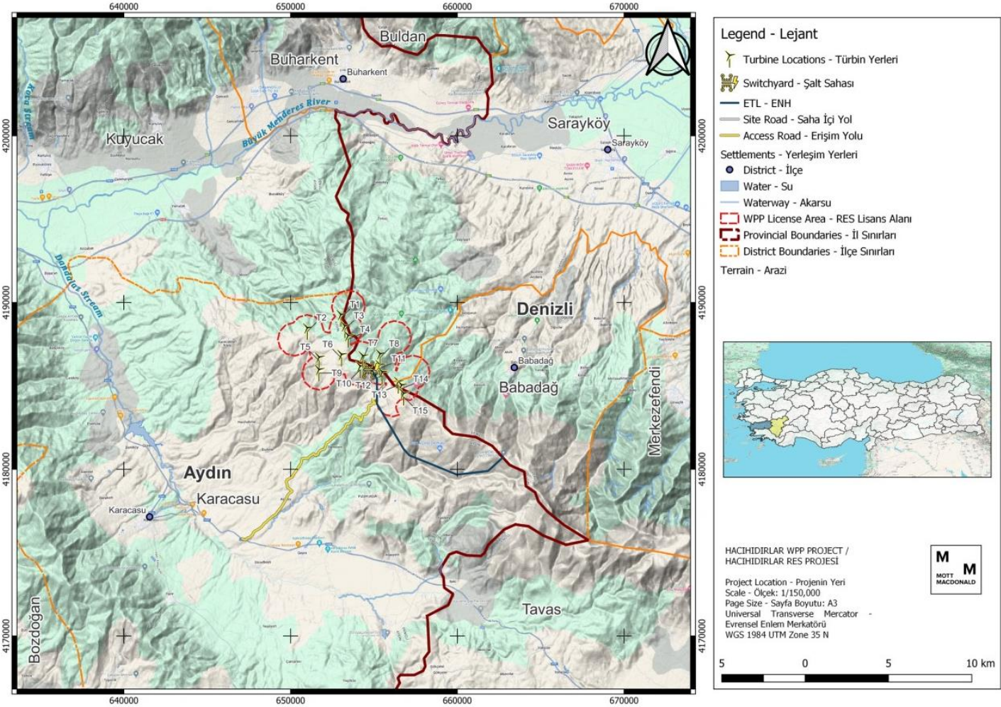
Figure 2.2: The Project Components Including the Access Roads and ETL
