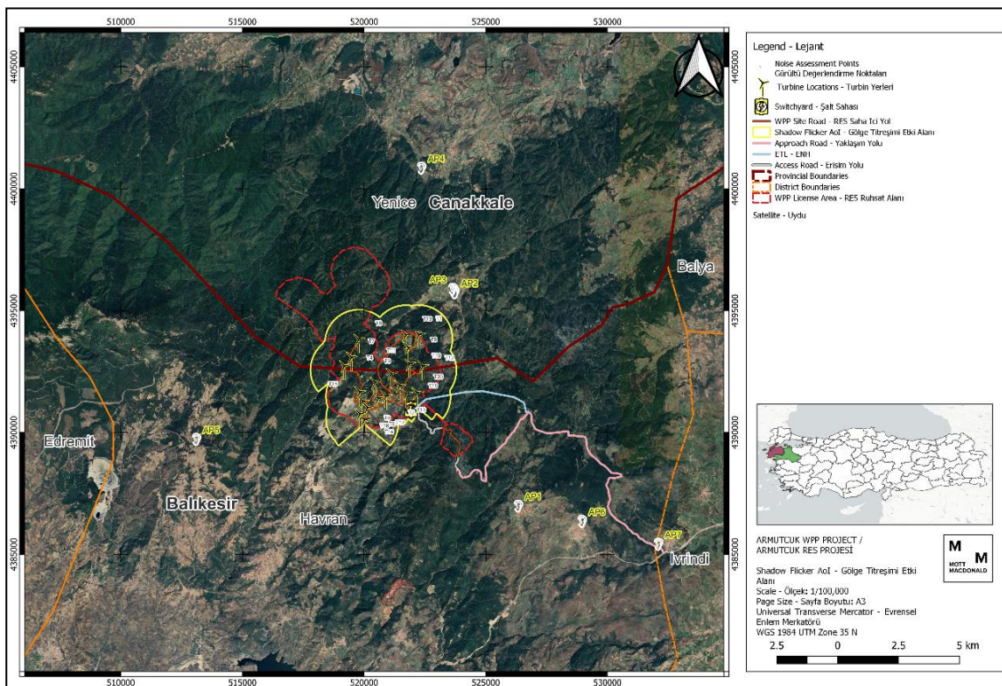
Figure 3.3: Shadow Flicker Aol ( \theta=260^\circ )
